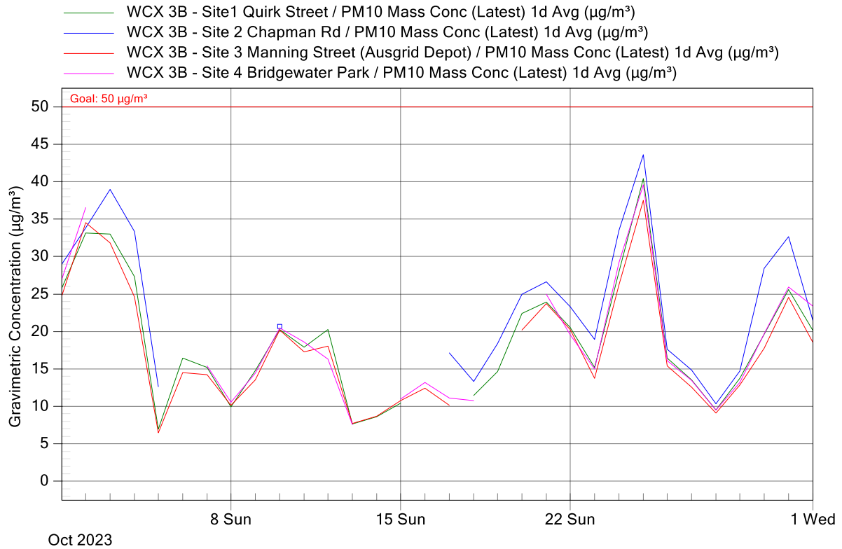
Figure 4: WCX 3B Project Air Monitoring Stations - PM 10 24-Hour Averages Graph for October 2023
