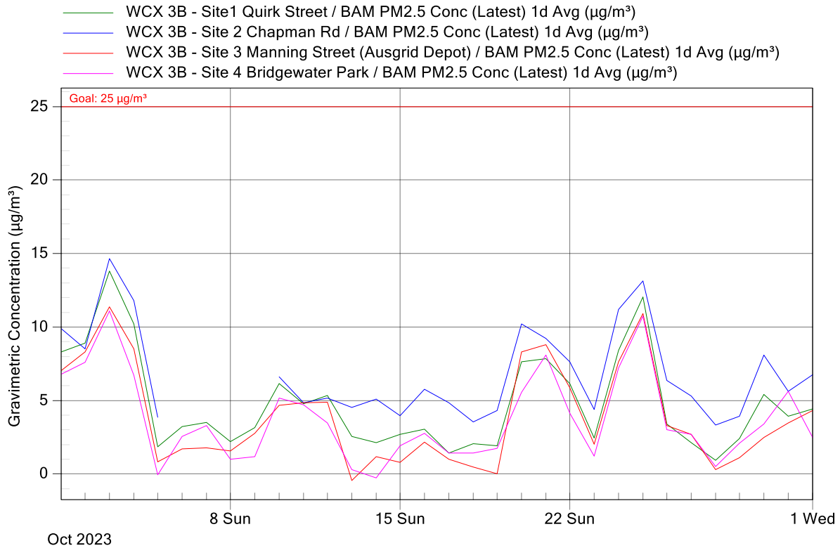
Figure 5: WCX 3B Project Air Monitoring Stations - PM 2.5 24-Hour Averages Graph for October 2023
