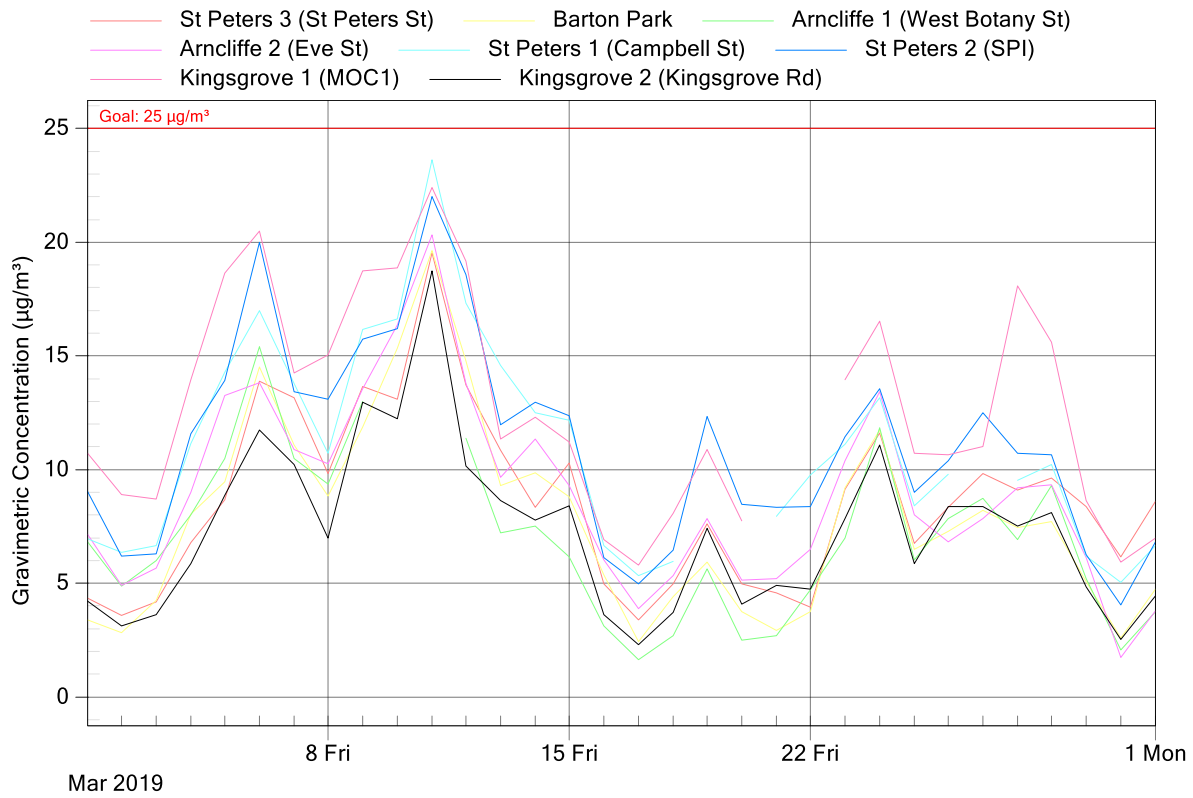
Figure 5: New M5 Project Air Monitoring Stations - PM 2.5 24 Hour graph March 2019
