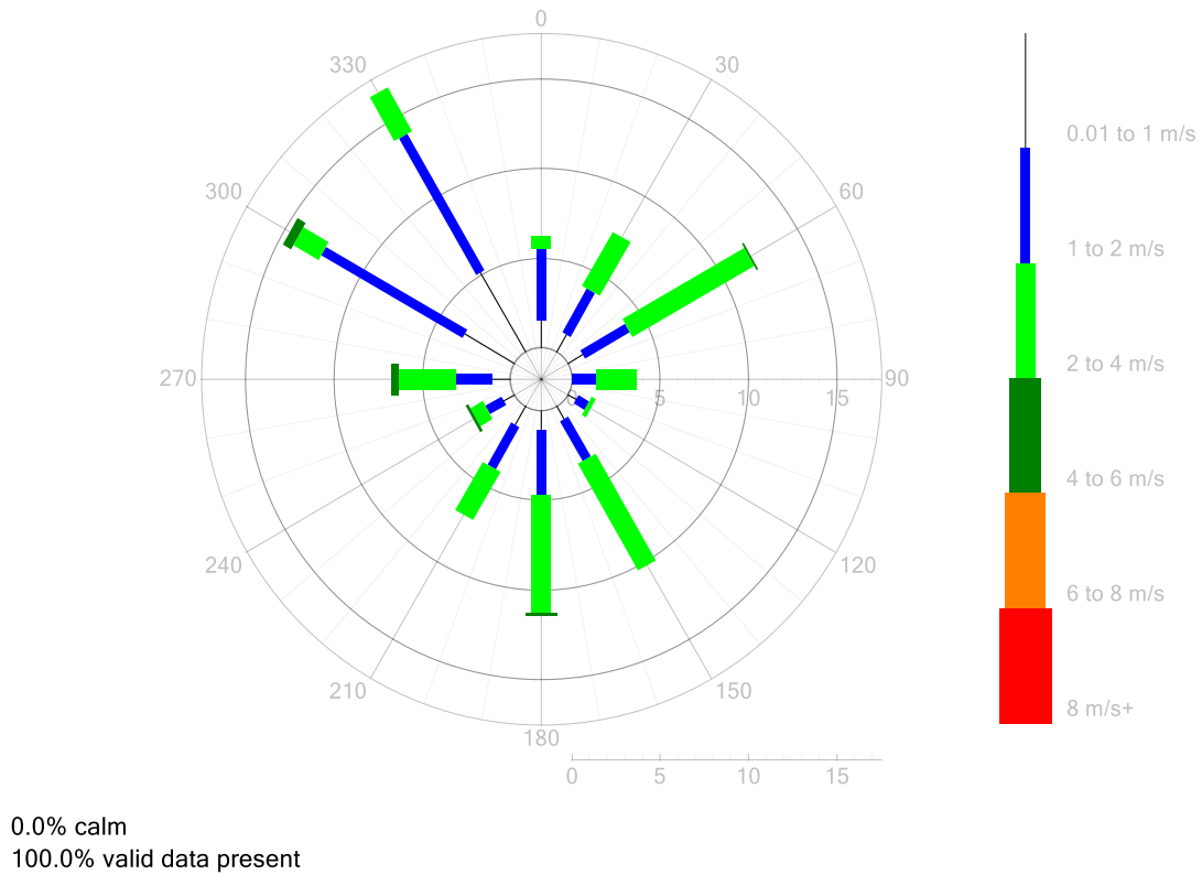
Arnccliffe 1 (West Botany St) - Wind Rose (1-hour average) Wind Rose March 2019
