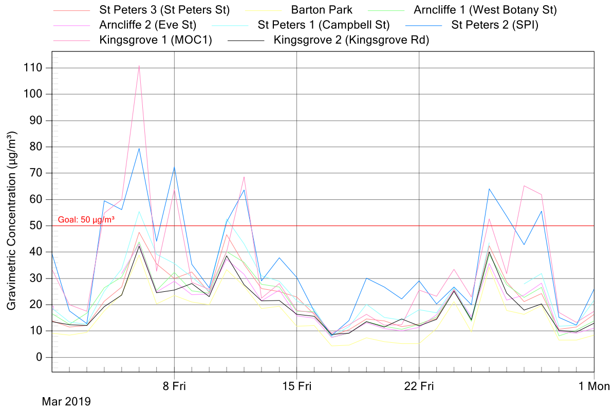
Figure 4: New M5 Project Air Monitoring Stations - PM 10 24 Hour graph for March 2019
