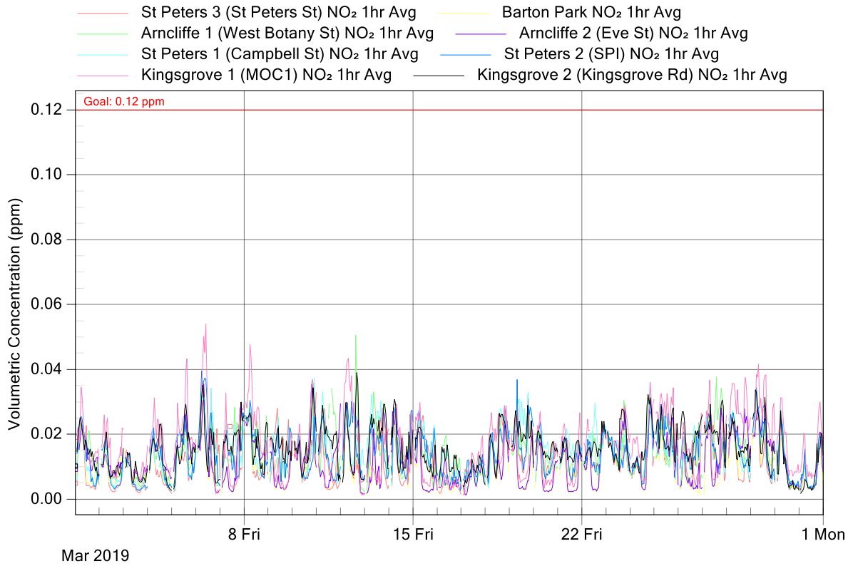
Figure 3: New M5 Project Air Monitoring Stations - NO 2 graph for March 2019
