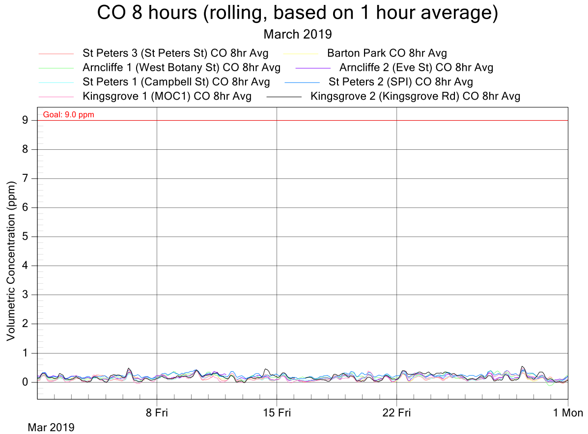
Figure 2: New M5 Project Air Monitoring Stations - CO 8 hours rolling graph for March 2019
