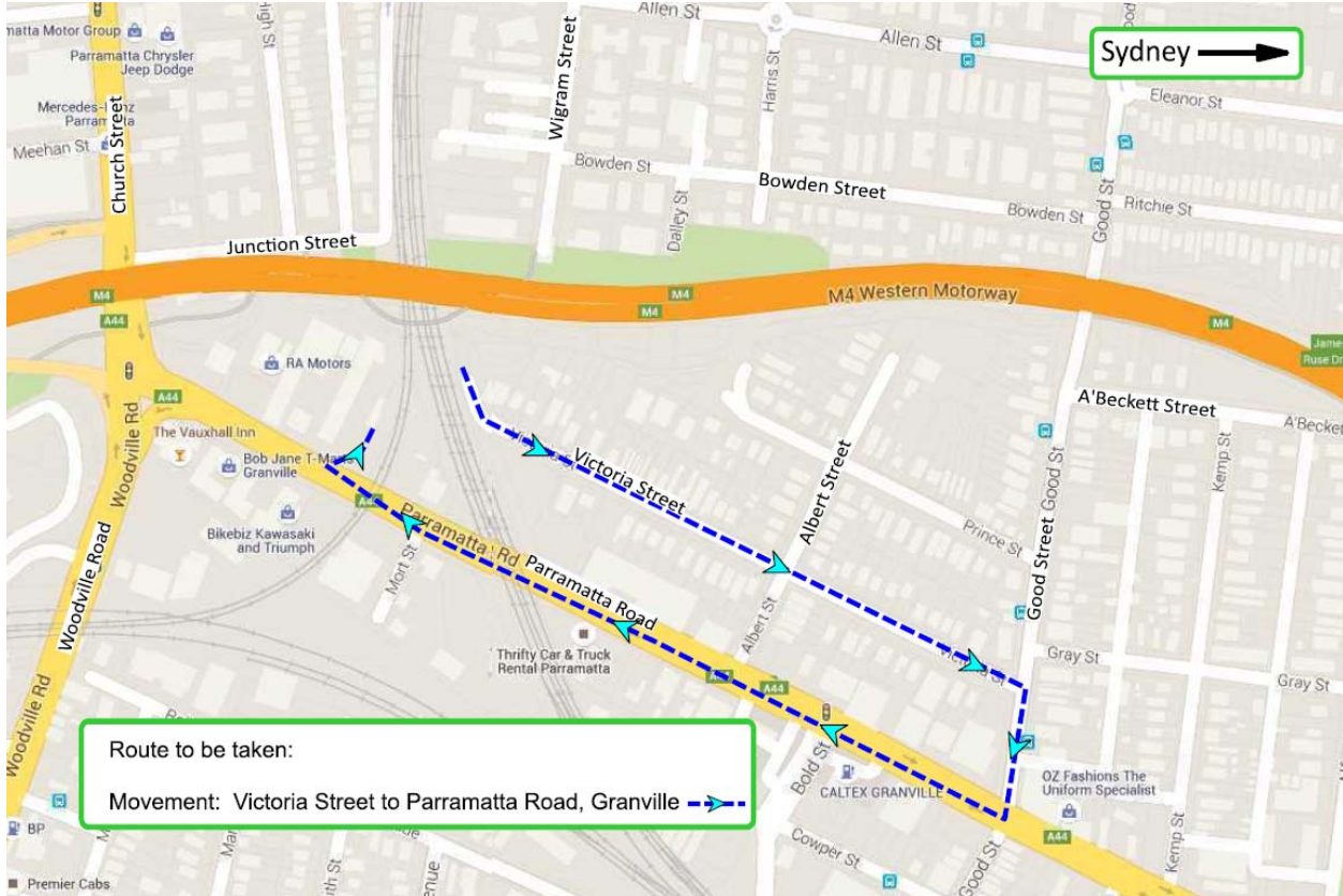
Figure 1 – Piling rig and crane movements from Friday, 5 February 2016
